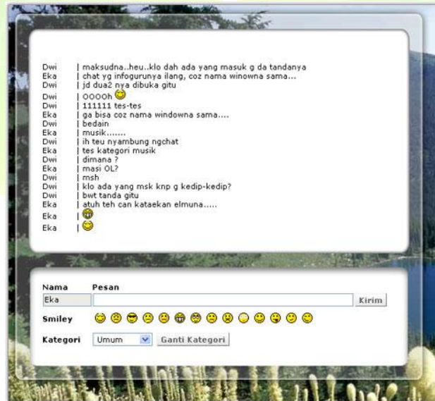
Gambar 18. Menu Chatting
